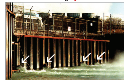
Water discharge area at the Palisades nuclear power plant on Lake Michigan. Note the flow from four big ejection outlets .
